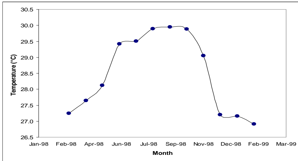
Figure 11: Temperature data at Gladden Spit, Belize
